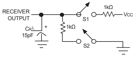
Figure 4. Receiver Timing Test Load
