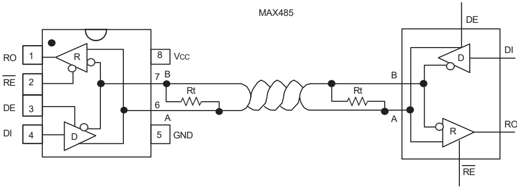
Figure 2. Typical Circuit
