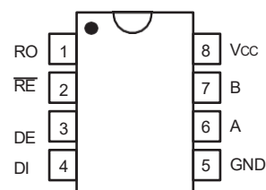
D OR P PACKAGE (Top View)
