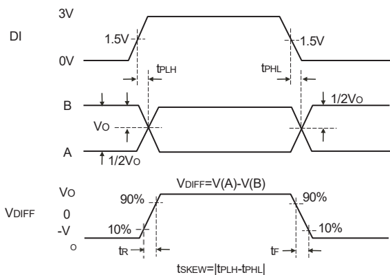
Figure 7. Driver transmission Delay timing
