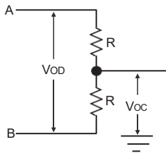
Figure 3. Driver DC Test Load
