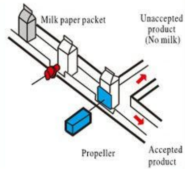
Capacitive type proximity switch
